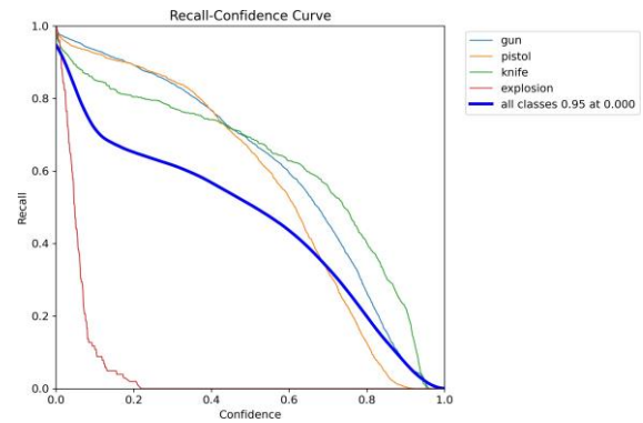
Figure 4.4: YOLOv8s Recall Curve
