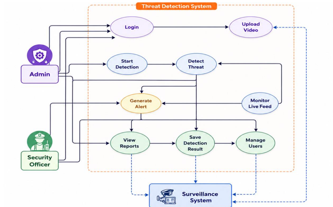
Figure 3.2: Use Case Diagram - YOLO Threat Detection.
