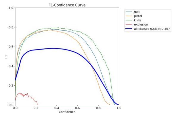
Figure 4.6: YOLOv8s F1 Score Curve
