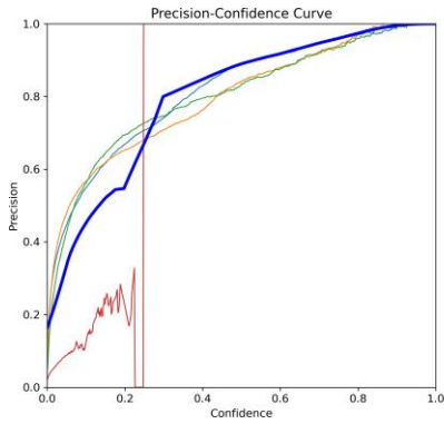
Figure 4.1: YOLO11s Precision Curve Figure 4.2: YOLOv8s Precision Curve The models have high precision at low confidence levels as demonstrated in Figure 4.1 and Figure 4.2. The gun and pistol detection accuracy of YOLO11s is better than other models, and other models still have excellent accuracy in all other classes.
