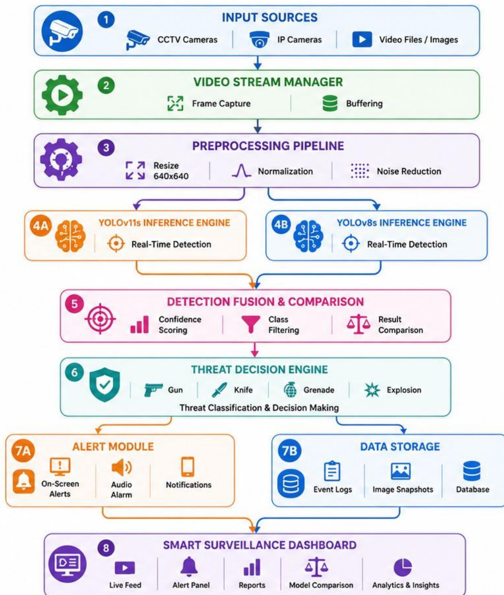
Figure 3.1: System Architecture - YOLO Threat Detection.
