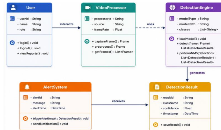
Figure 3.3: UML Class Diagram - YOLO Threat Detection (Visual Style).
